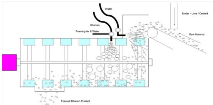
Figure 2 Material flow through the pugmill, showing the incorporation of foamed bitumen via the spray-bar.
