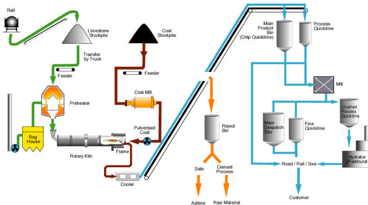
Figure 2 Lime manufacturing plant. (Diagram courtesy of Pacific Lime)
