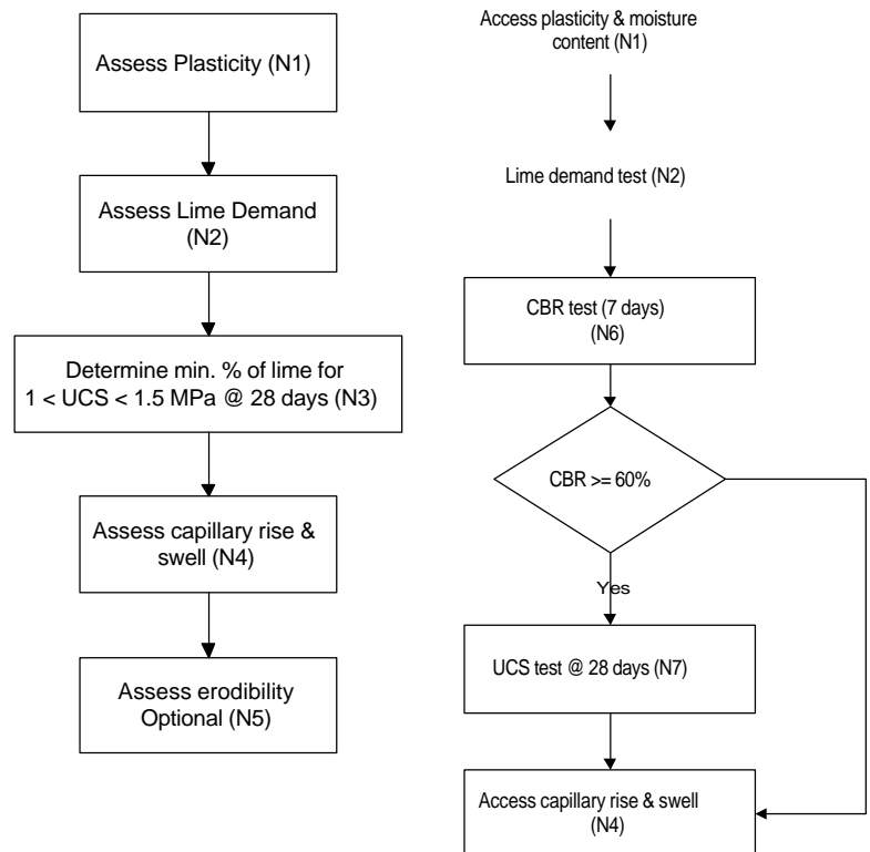
Figure 3 Lime content using the UCS and CBR approaches [Ref.3].
